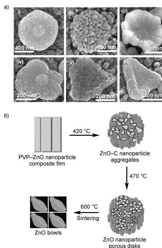
Figure 4. Extraction of intermediate morphologies for different calcination times at 470 °C: a) Emergence of bowl- and troughlike morphologies from the bladelike ZnO–PVP composite. i, iv) Calcination of the composite at 470 °C for 1 h resulted in the formation of circular and triangular composite structures; ii, v) calcination at 470 °C for 5 h resulted in a porous morphology owing to the removal of the polymer; iii, vi) calcination at 470 °C for 8 h transformed these porous structures into zeptoliter bowls and triangular troughs. b) Schematic illustration of the formation of ZnO bowls.
