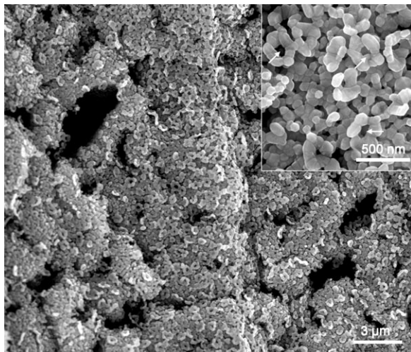
Figure 3. FESEM image of corrugated ring-shaped ZnO nanostructures: Calcination of the ZnO–PVP composite at 600 °C for 1 h duration with a faster rate of heating (20 °Cmin −1 ) resulted in the formation of ZnO rings. Each of these rings is further made up of 10 to 12 ZnO nanoparticles of approximate sizes 50 to 80 nm; inset: magnified image of these rings with arrows pointing towards the holes.
